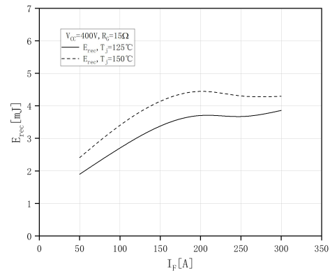
开关损耗二极管(D5, D6), 逆变器 (典型) Switching losses Diode(D5, D6), Inverter(typical)
