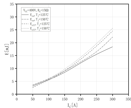
开关损耗 IGBT(Q2, Q3), 逆变器 (典型) Switching losses IGBT(Q2, Q3), Inverter (typical)
